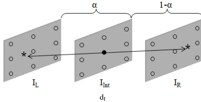
Figure 3.1: Shows backward-disparity estimation (disparity compensation from intermediate disparity to the left and right disparity)
