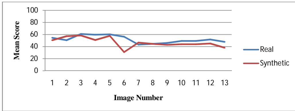
Figure 7.17: Mean of difference scores for the forward algorithm under different types of images
